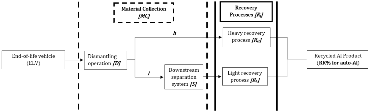
Figure 3: Automotive aluminum material flow model: grave-to-gate (auto-aluminum parts at a dismantling yard to a recycled Al product).
