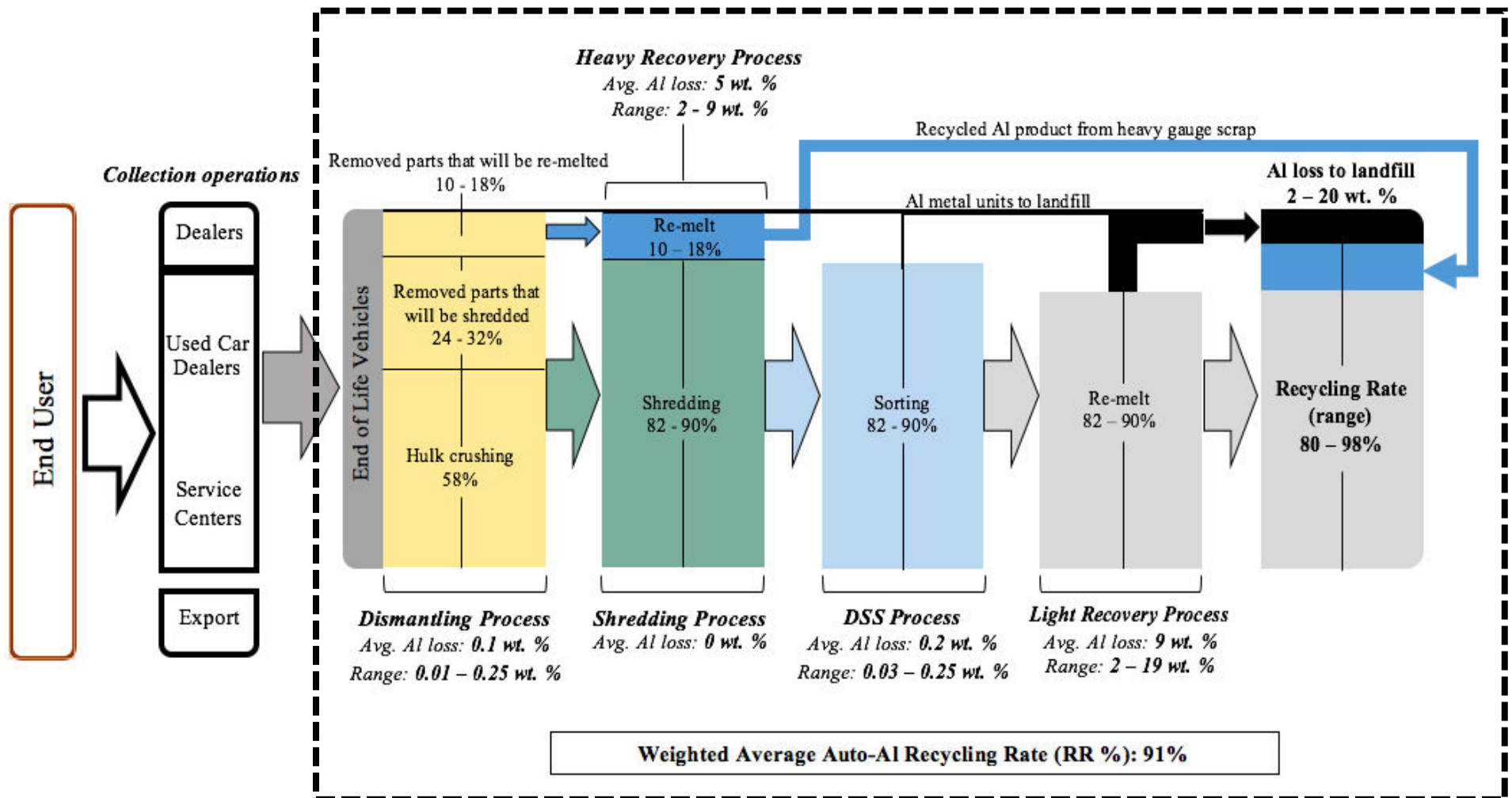
Figure 4: Process material flow analysis for automotive aluminum.
