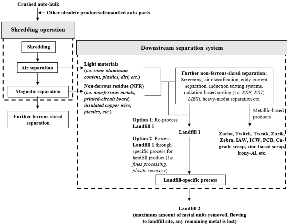
Figure 2: Shredding operation and downstream separation system definitions.
